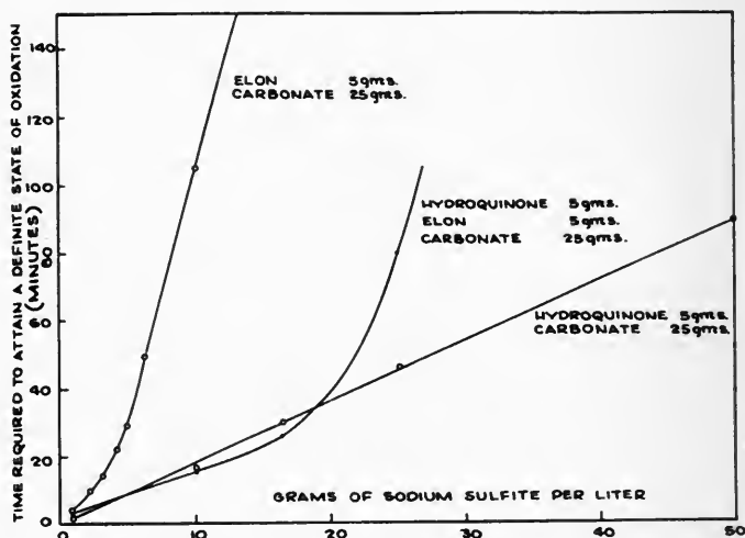
FIG. 7. Effect of sulfite concentration on the rate of oxidation of developers containing (a) elon, (b) hydroquinone, and (c) mixtures of elon and hydroquinone.
